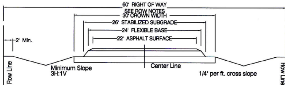
TYPICAL ROADWAY SECTION
