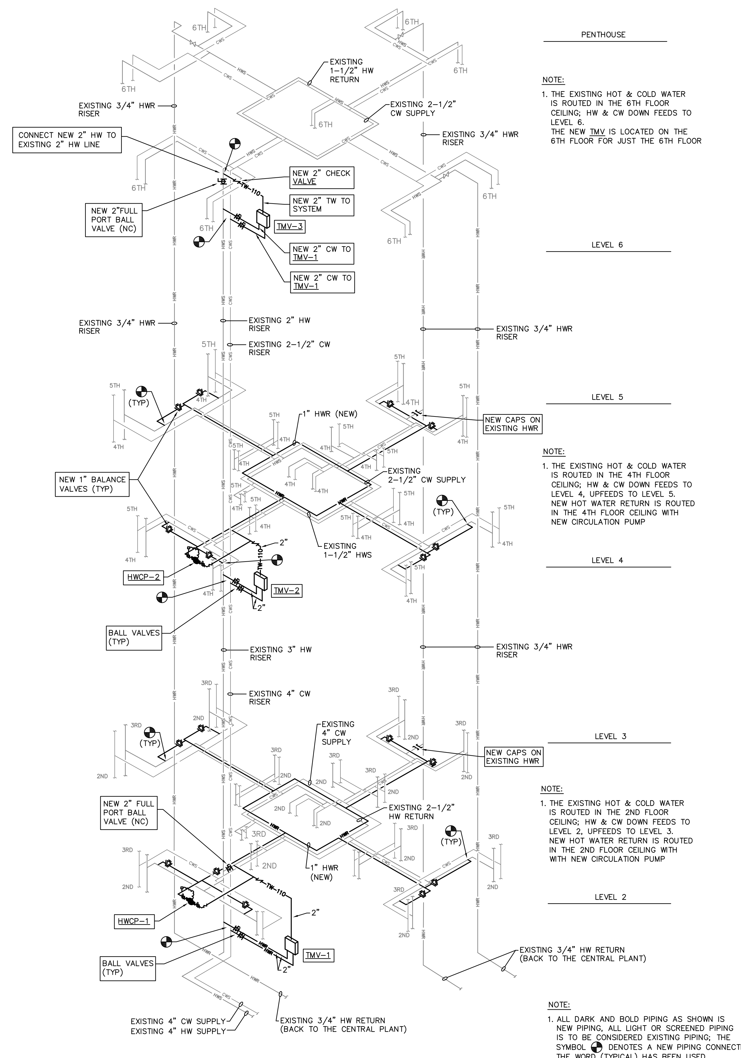
1 HOT WATER RISER DIAGRAM SCALE: NONE
