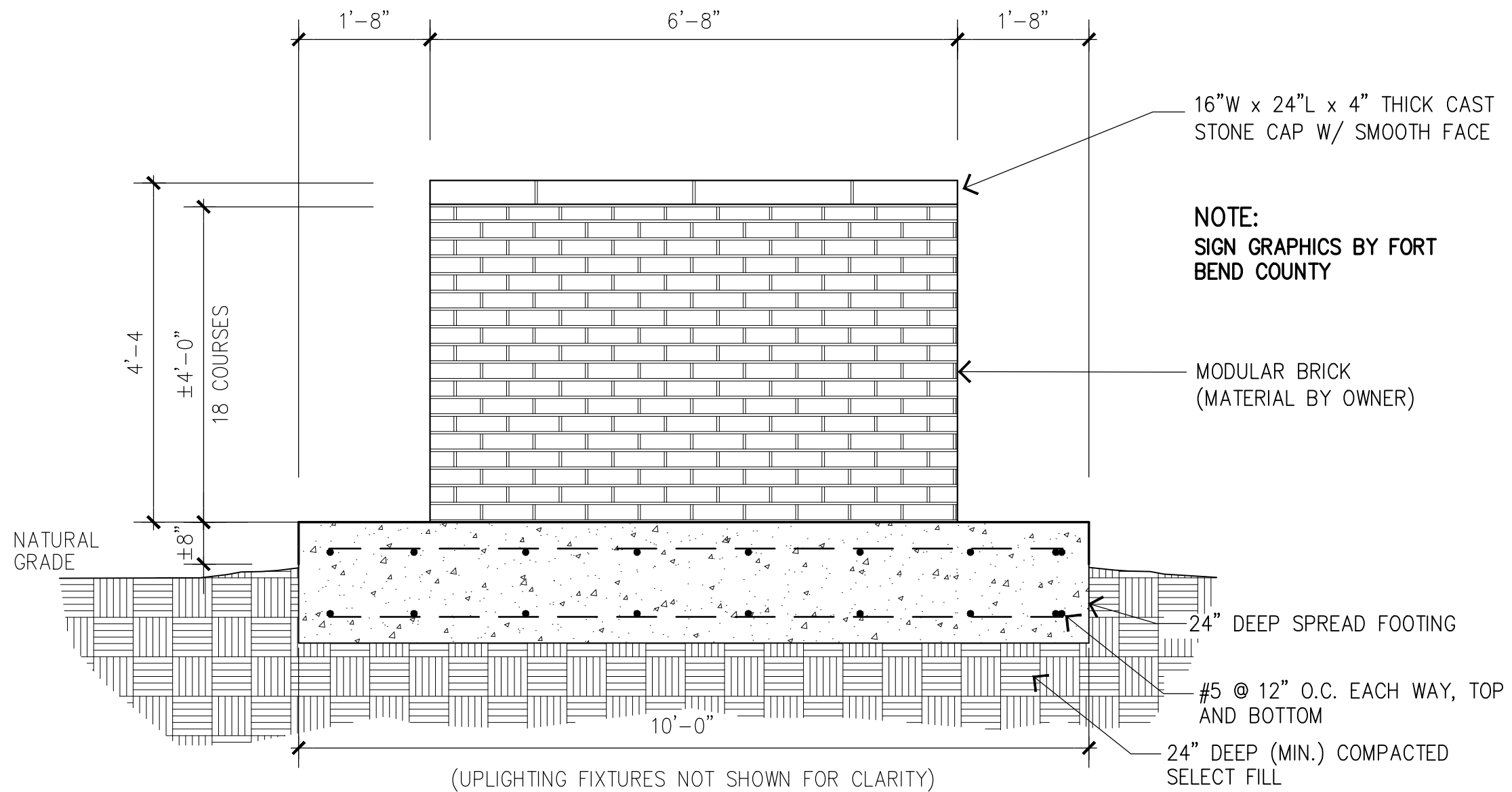
FRONT ELEVATION
