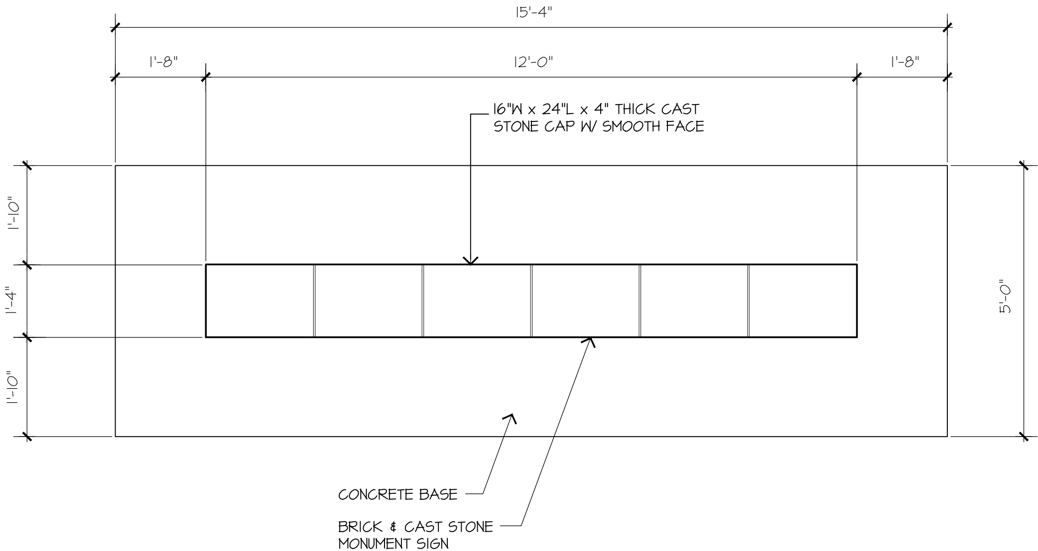
PLAN VIEW
