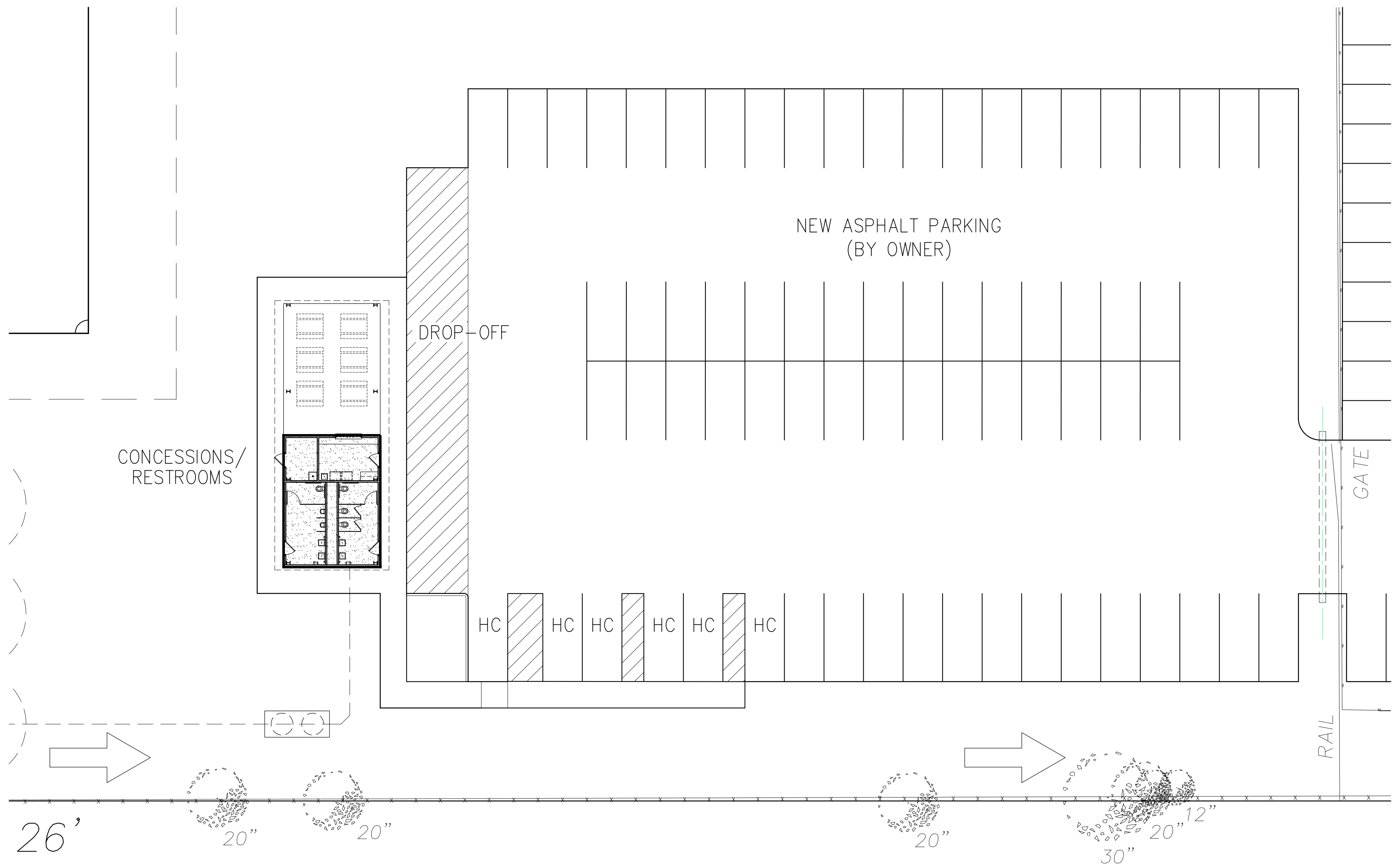
SITE PLAN CONCESSIONS/RESTROOMS
